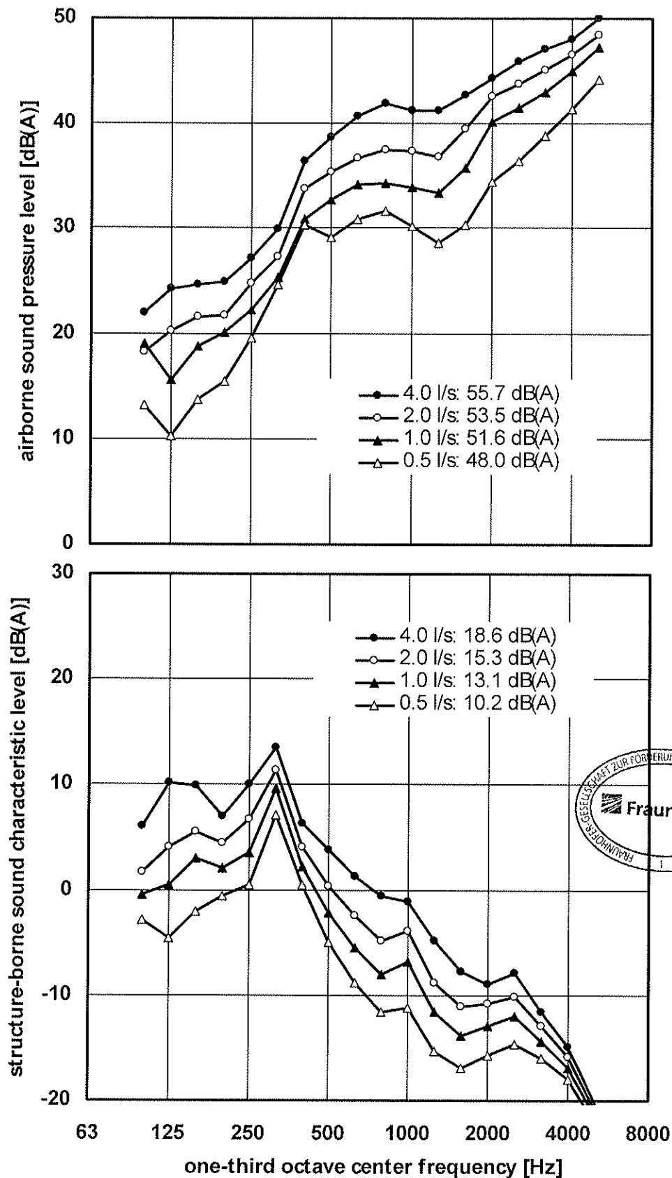
Figure 2 Wastewater pipe system "Ultra Silent 110 x 3.4" mounted according to figure 4, using pipe clamps "Müpro yellow, with spacer 5 mm". Airborne sound pressure level (above) and structure-borne sound characteristic level (below) measured at various flow rates according to DIN EN 14366.
