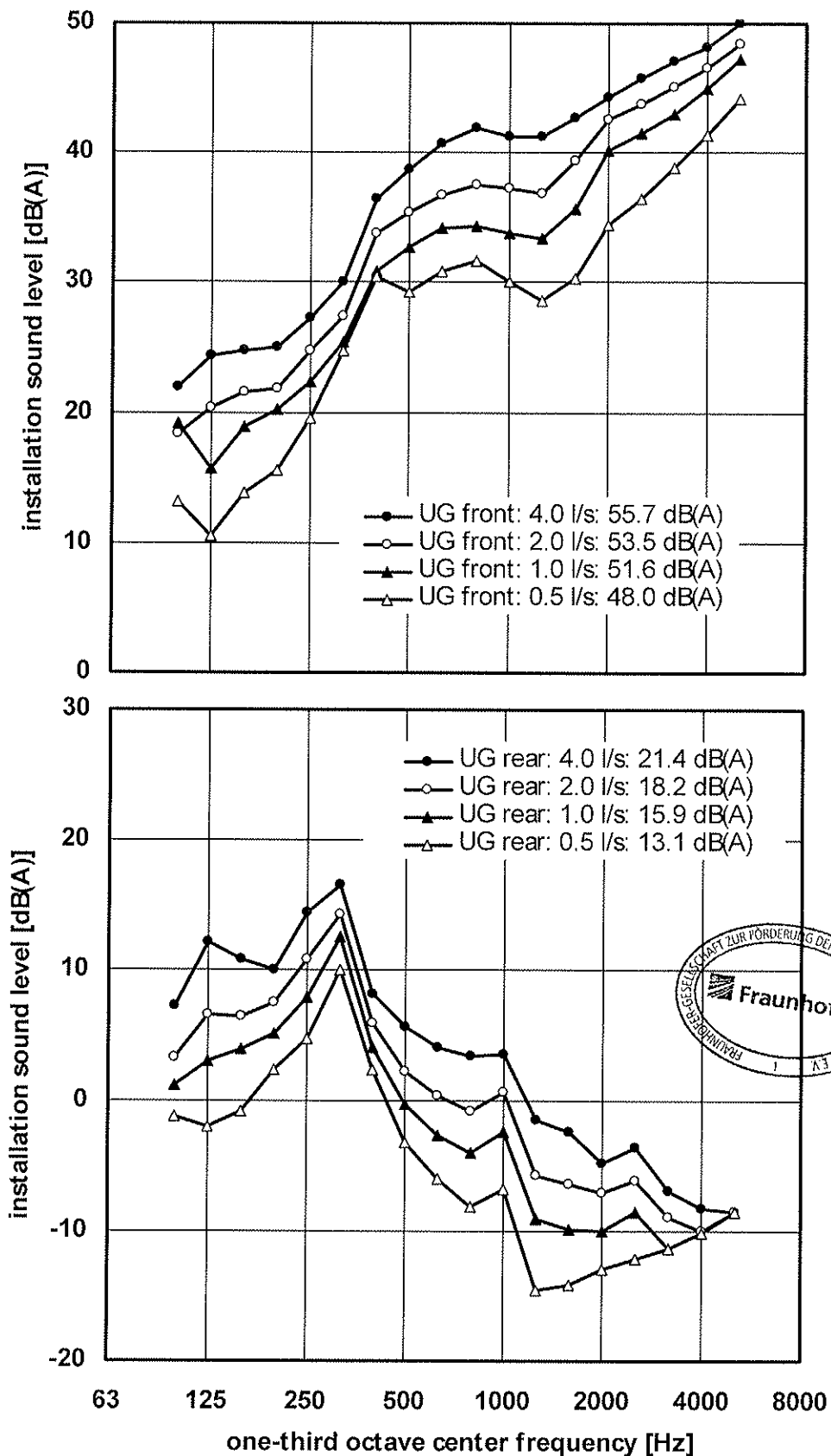
Figure 1 Wastewater pipe system "Ultra Silent 110 x 3.4" mounted according to figure 4, using pipe clamps "Müpro yellow, with spacer 5 mm". The installation sound level L_{in} was measured at various flow rates in the test rooms UG front (above) and UG rear (below).
